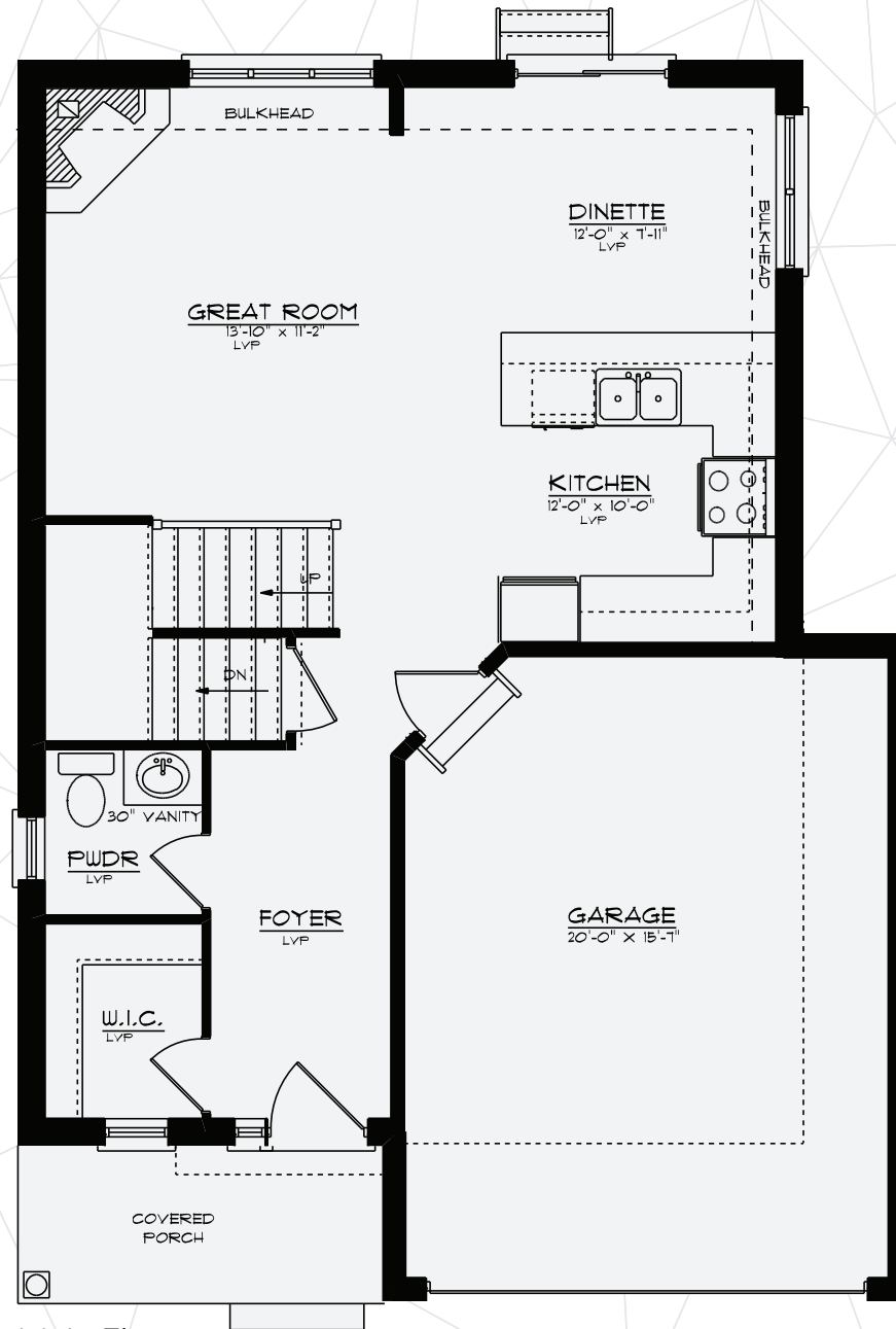
Main Floor 690 Sq. Ft.
