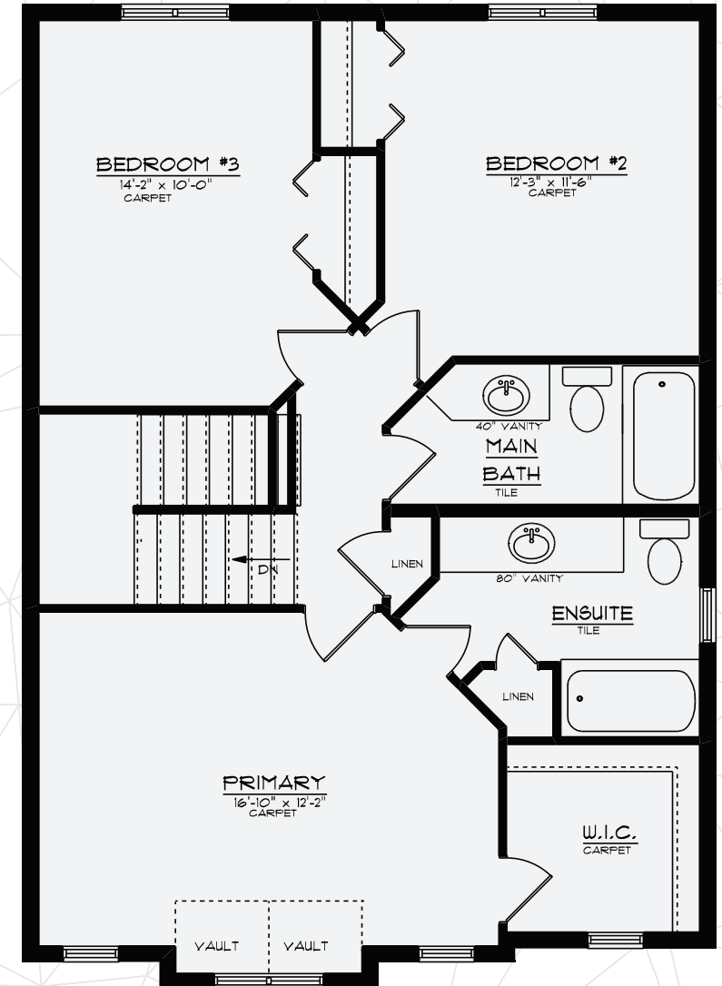
Upper Floor 891 Sq. Ft.
